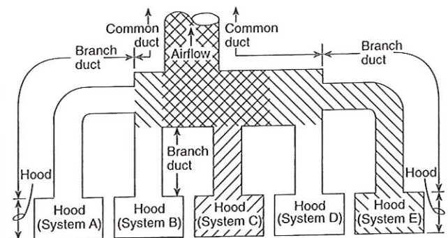
FIGURE A.9.3.4.1(2)(b) Simultaneous Operation of Two Systems in Which One Also Provides Common Duct Protection.
