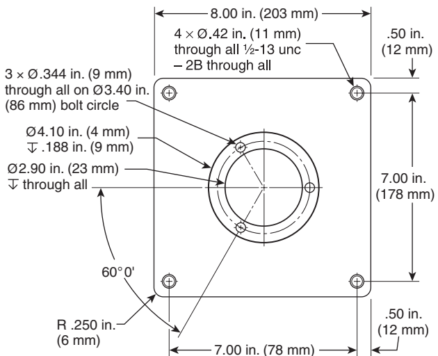
FIGURE B.19(e) Base Support Plate, ⅜ in. (10 mm) Thick.
