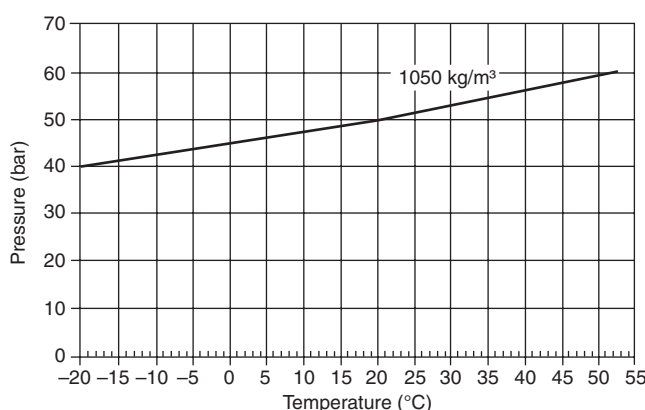
(6) HFC-227ea pressurized to 50 bar at 20°C
