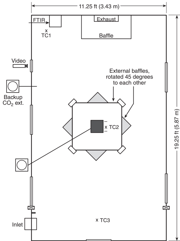
FIGURE A.5.4.2.2(a) Four Piece Modified Plastic Setup.
