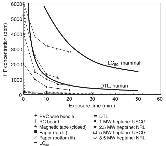
FIGURE A.5.7.1.1(b) Hazard Assessment of HF Concentrations. Extinguishment of Typical EDP and Class B Hazards with 7 Percent HFC-227ea.
