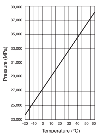
(6) Pressurized to 30.0 MPa at 15°C
