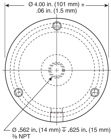
FIGURE B.19(d) Base, Detail.
