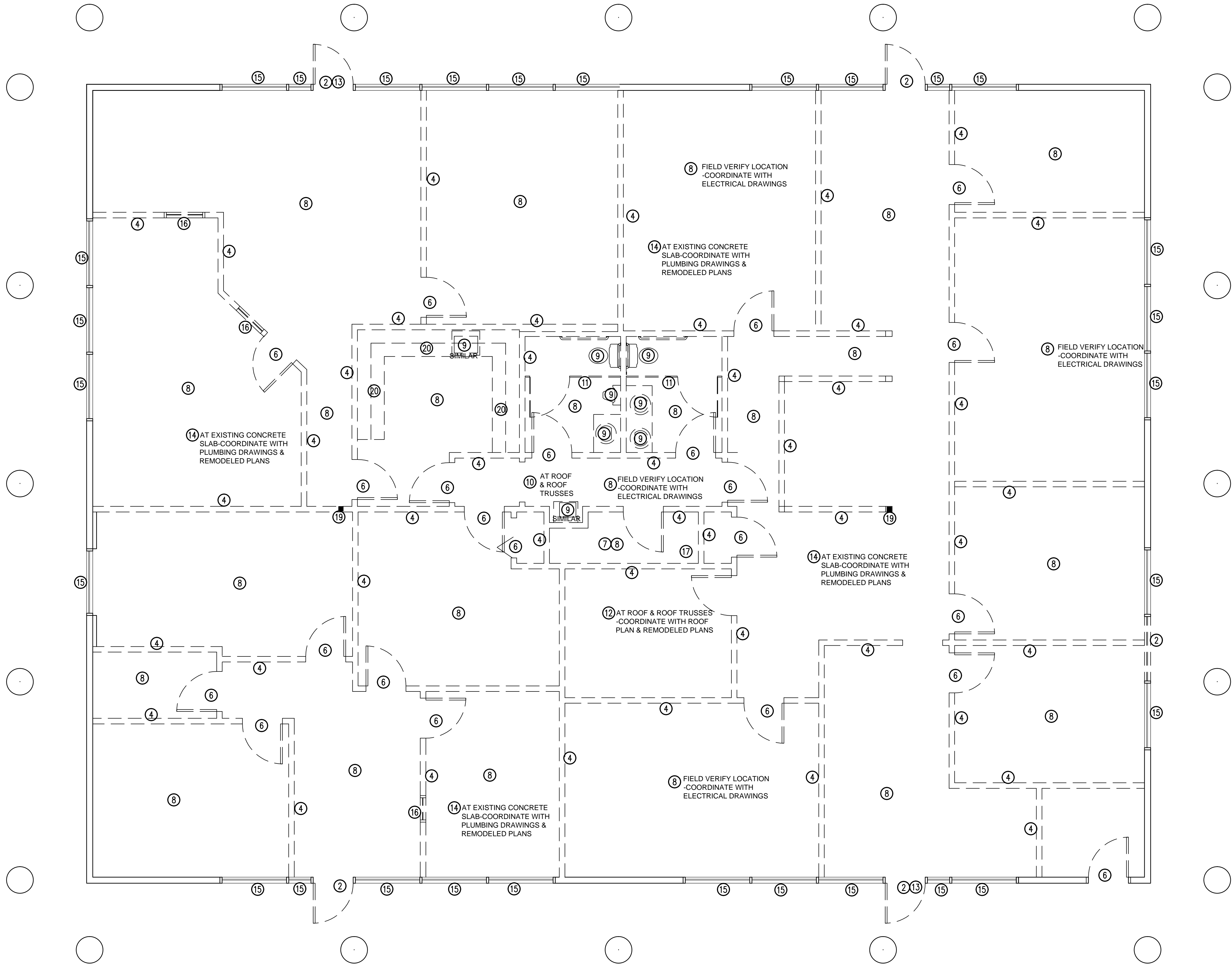
EXISTING DEMOLITION FLR .PLAN-BUILDING 'A' SCALE: 1/4" = 1'-0"
