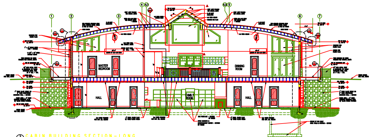
2 CABIN BUILDING SECTION-LONG 1/8" = 1'-0"
