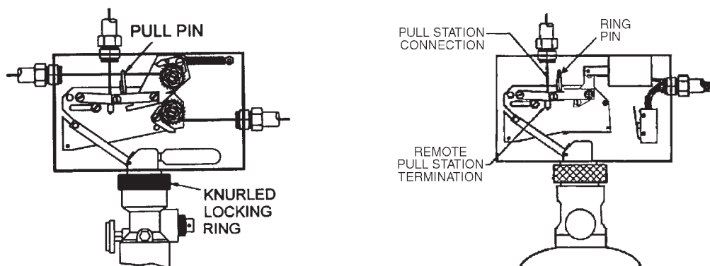
Figure 4-2. Single Cylinder Installation Using Model MCH3/ECH3 Control Head.
