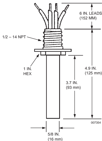
Figure 2-12a. Thermal Detector.
