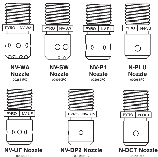
Figure 2-3 Nozzles
