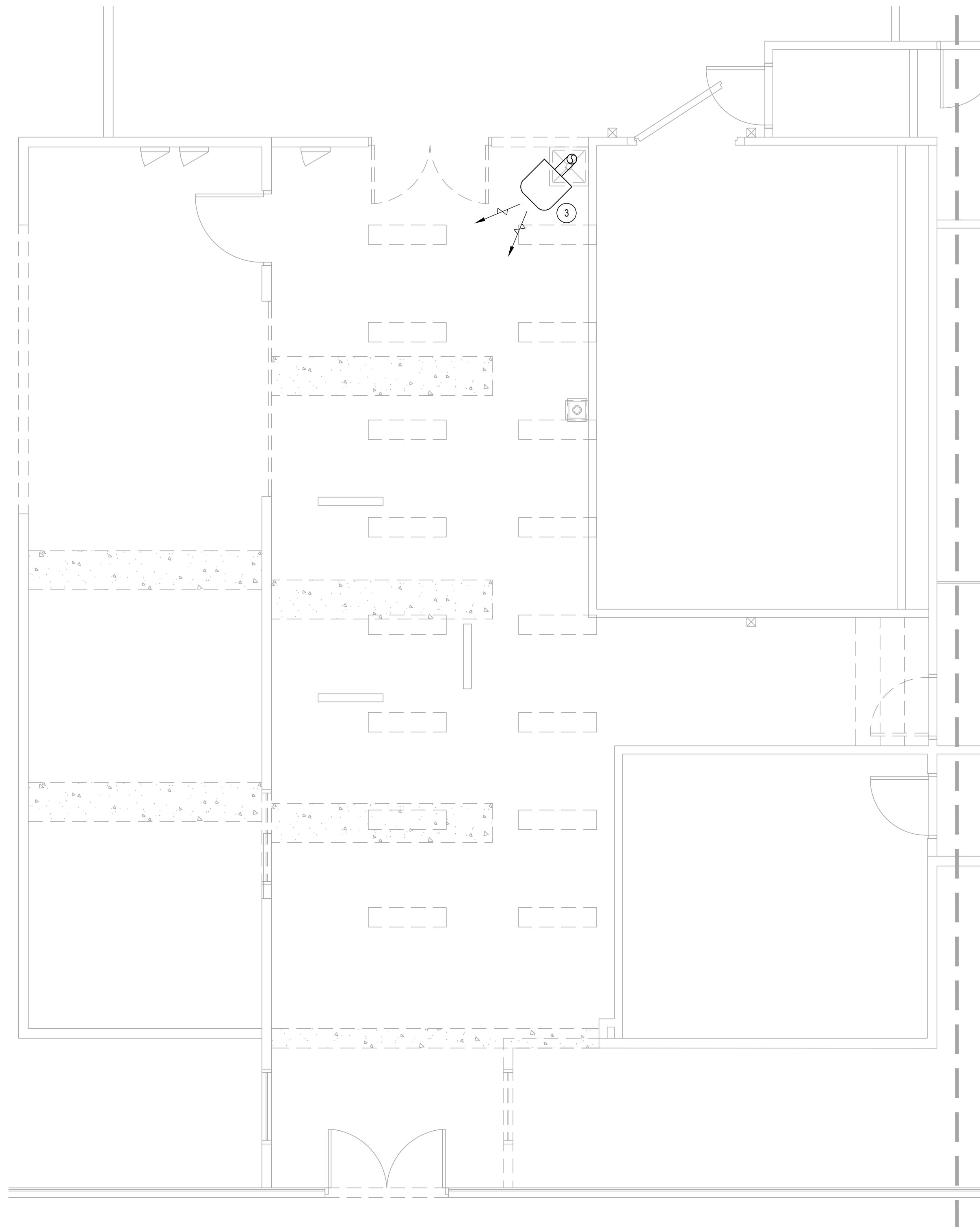
NORTH MECHANICAL DEMO PLAN SCALE: 1/4"=1'-0"
