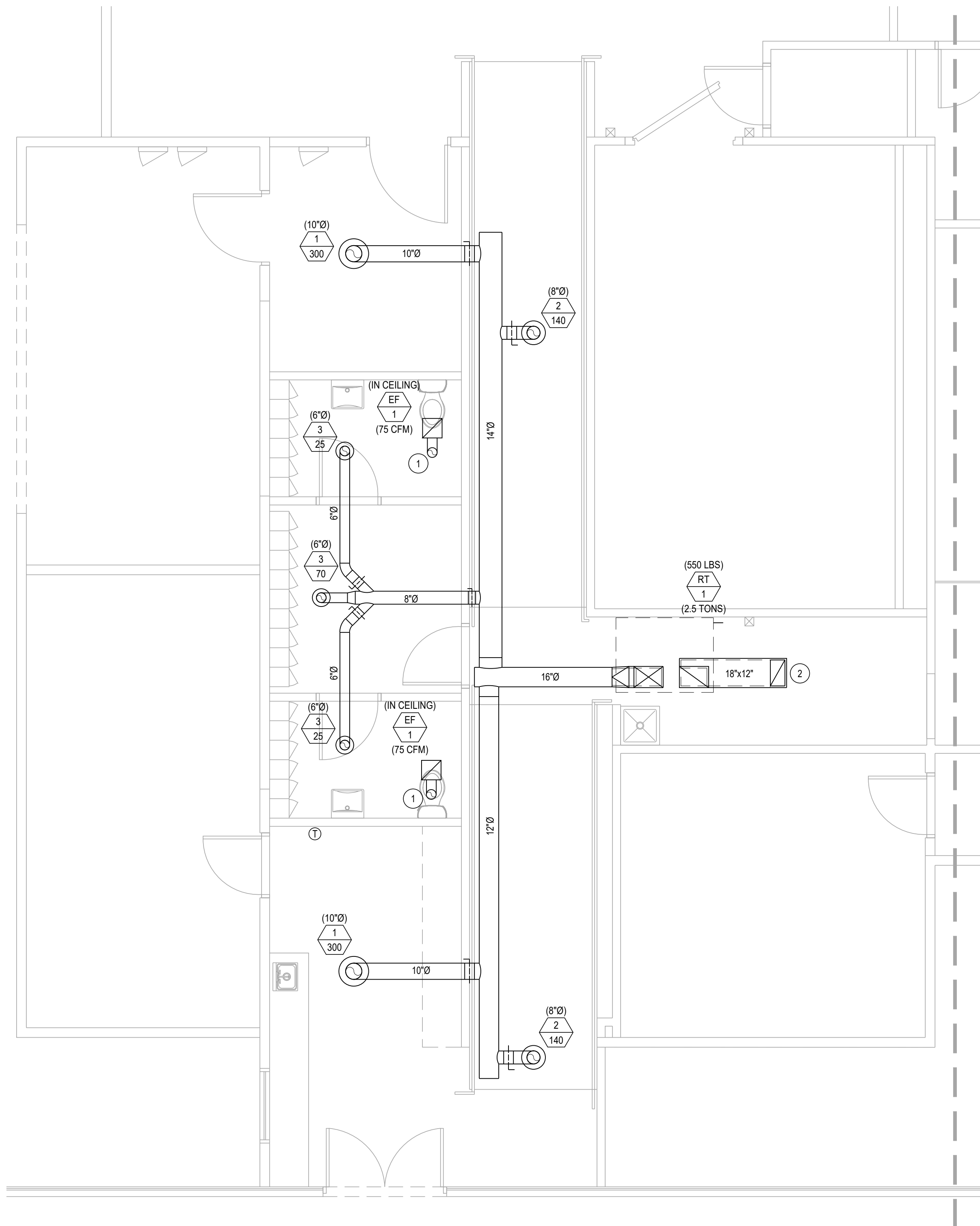
NORTH MECHANICAL PLAN SCALE: 1/4"=1'-0"
