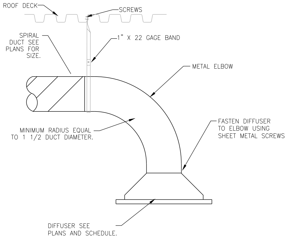
B DUCT MOUNTED DIFFUSER DETAIL NTS
