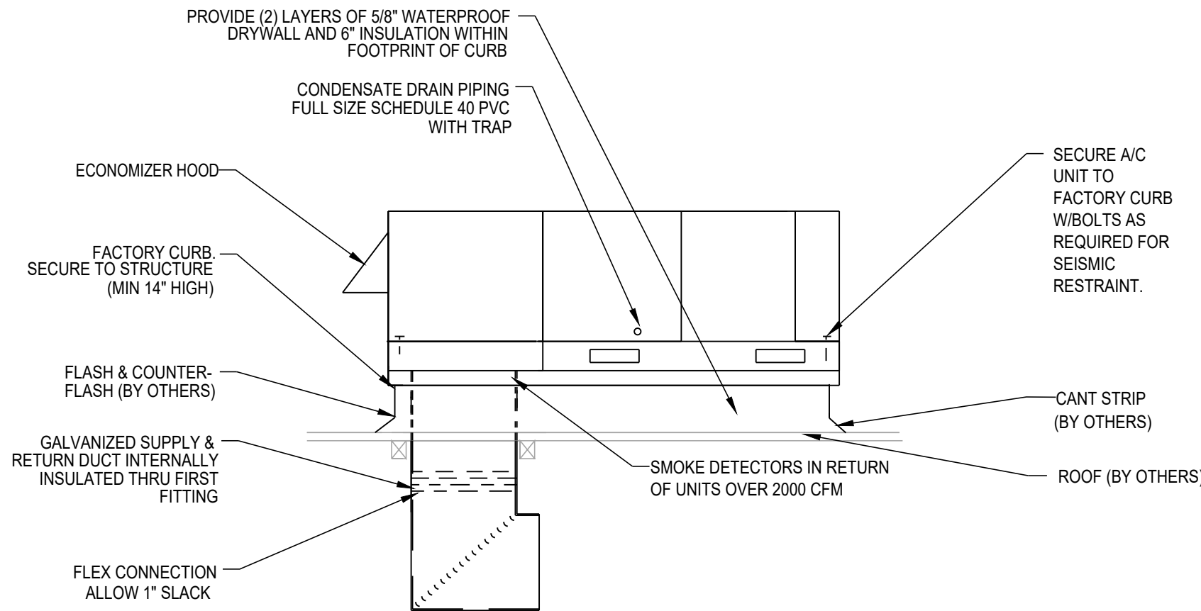
D PACKAGED ROOFTOP UNIT DETAIL NTS
